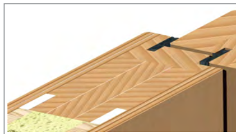
Detail: ISOCORE-Tech Türblatt Rohling
